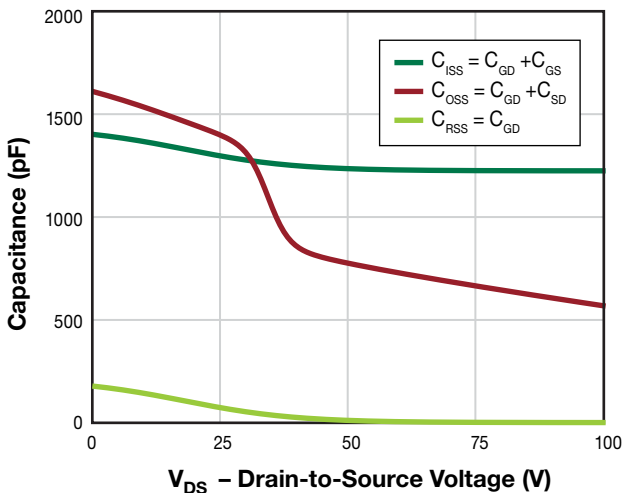
Figure 11. Typical Capacitance
