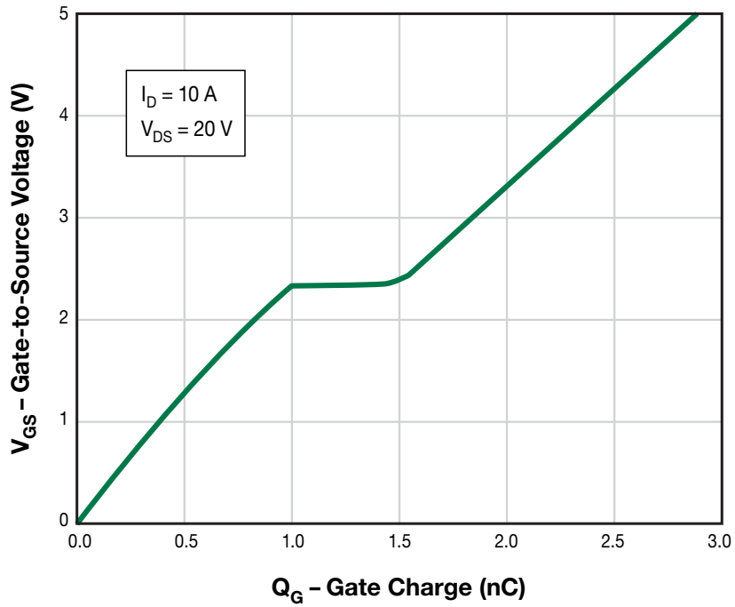
Figure 13. Typical Gate Charge
