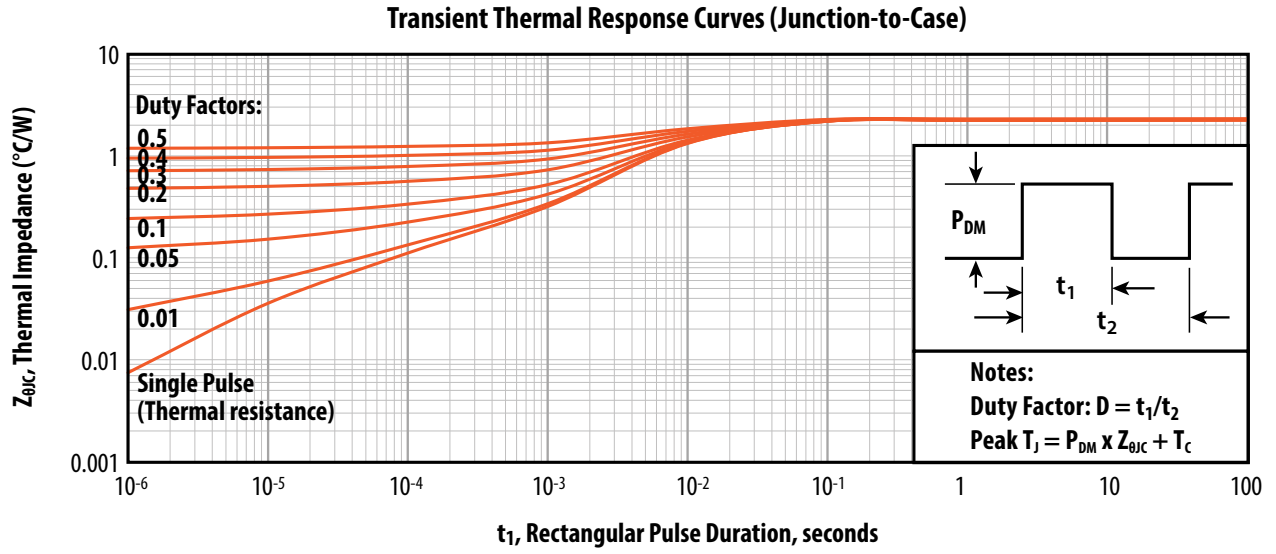
Figure 15. Transient Thermal Impedance, Junction to Case
