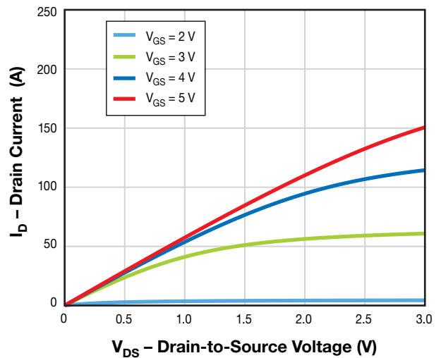
Figure 4. Typical Output Characteristics at 125 °C
