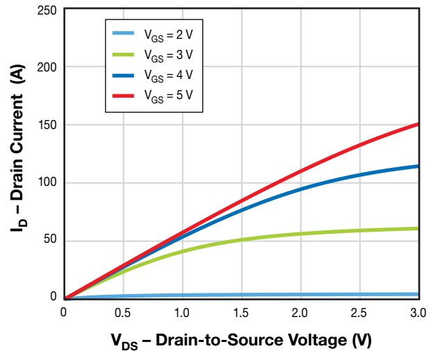
Figure 5. Typical Output Characteristics at 125 °C
