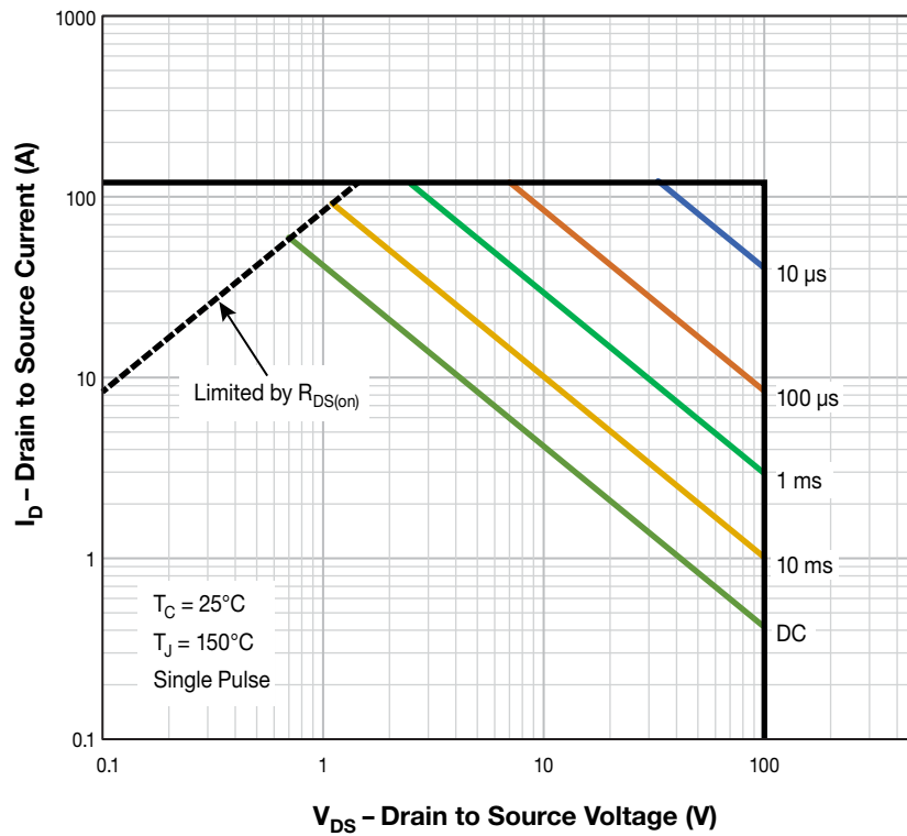
Figure 14. Safe Operating Area
