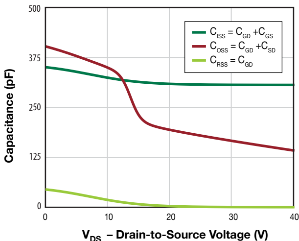
Figure 11. Typical Capacitance
