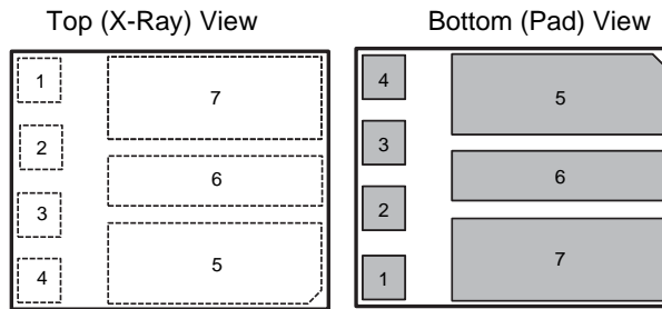
EPC7011L7BH Configuration and Pin Assignment Table
