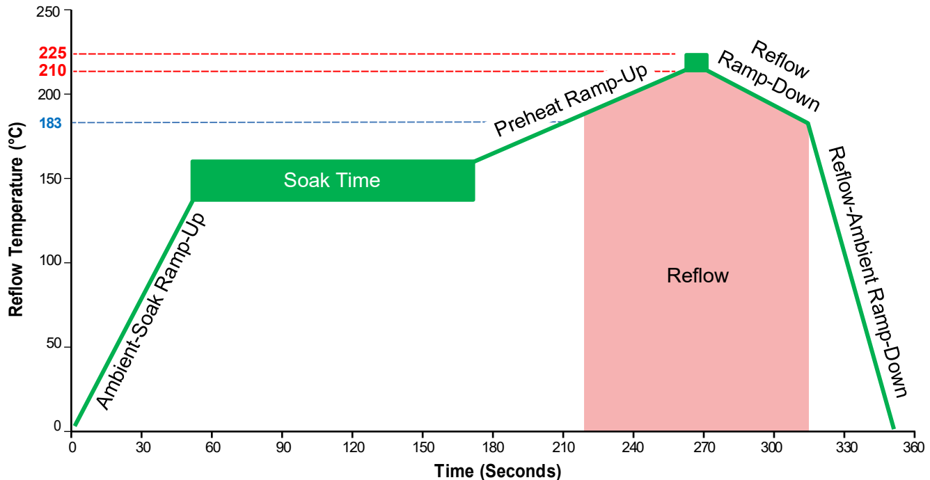
Figure 15. Typical EPC7011L7BH Package SN63/37 Solder Attachment Reflow Profile
