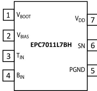
Figure 5. Suggested EPC7011L7BH Integrated Circuit Schematic Symbol
