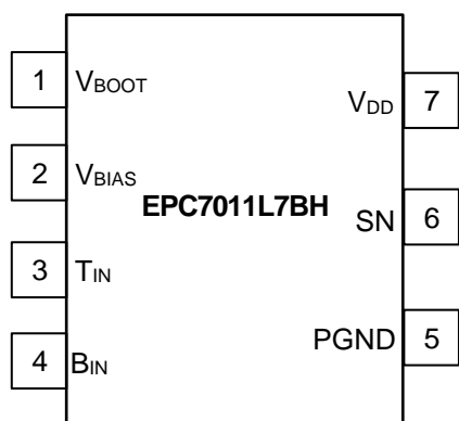
Figure 5. Suggested EPC7011L7BH Integrated Circuit Schematic Symbol
