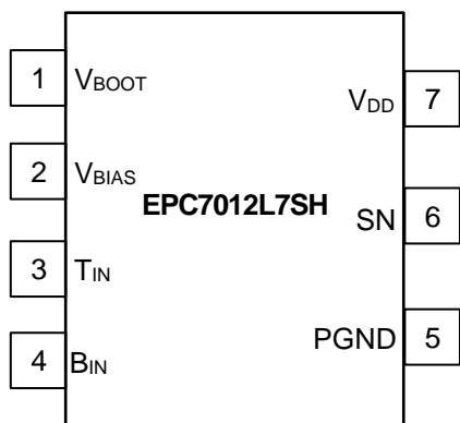
Figure 5. Suggested EPC7012L7SH Integrated Circuit Schematic Symbol
