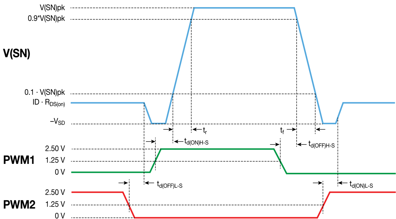
Figure 1. Switching Figures
