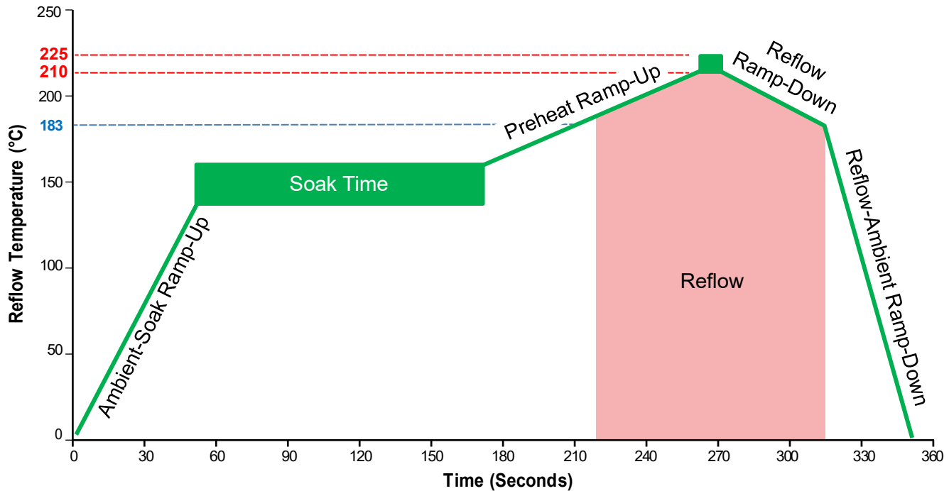
Figure 15. Typical EPC7012L7SH Package SN63/37 Solder Attachment Reflow Profile
