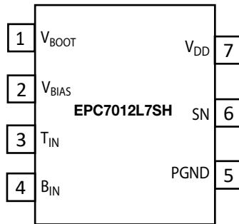
Figure 5. Suggested EPC7012L7SH Integrated Circuit Schematic Symbol
