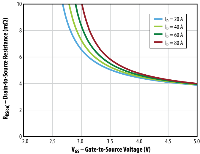
Figure 7: R_{DS(on)} vs. V_{GS} for Various Drain Currents
