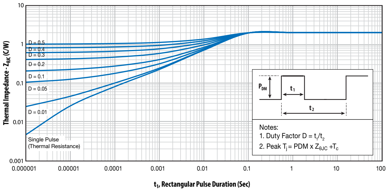
Figure 15: Thermal Impedance diagram
