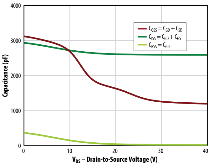
Figure 12: Typical Capacitance
