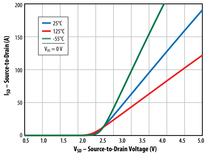
Figure 6: Reverse Drain-Source Characteristics
