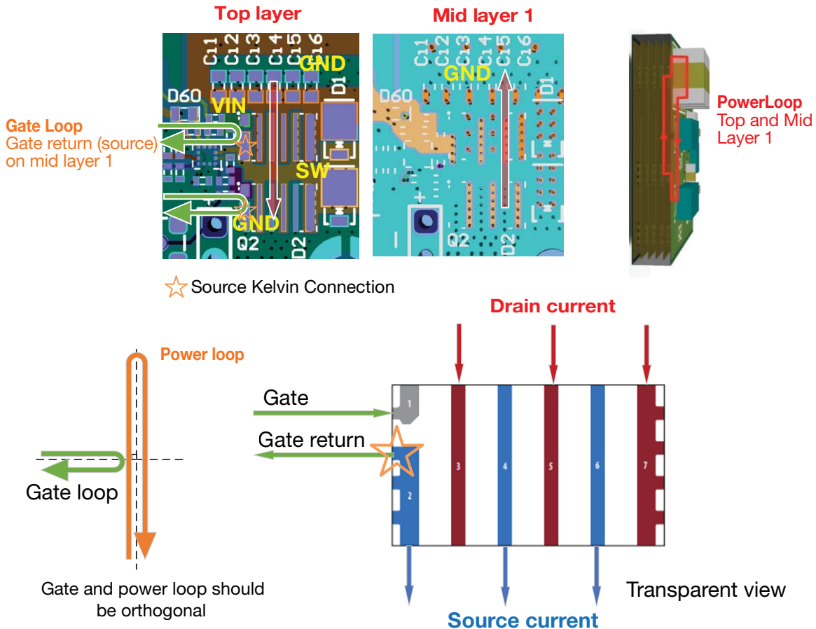
Figure 16: Inner Vertical Layout for Power and Gate Loops from EPC90133
