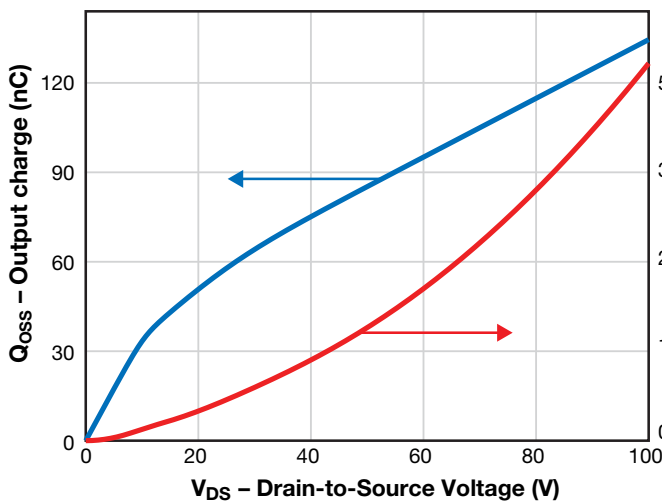
Figure 5: Typical Output Charge and C_{OSS} Stored Energy
