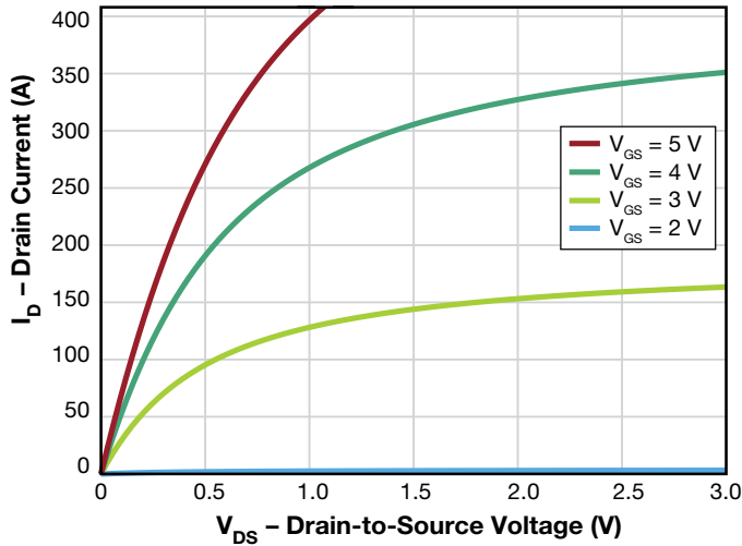
Figure 1: Typical Output Characteristics at 25°C
