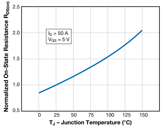
Figure 8: Typical Normalized On-State Resistance vs. Temperature
