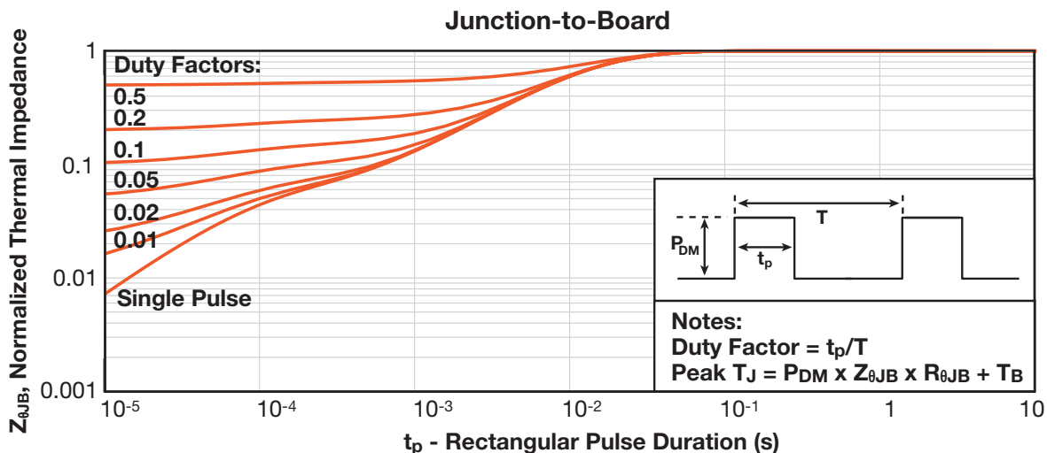
Figure 13: Typical Transient Thermal Response Curves
