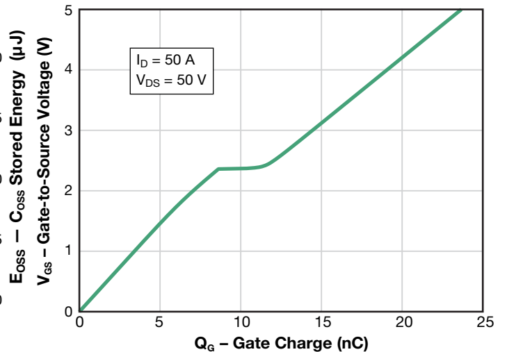
Figure 6: Typical Gate Charge
