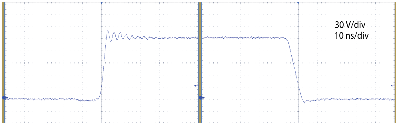
Figure 16: Typical half-bridge voltage switching waveforms
