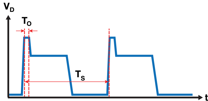
Figure 14: Duty Cycle Factor ( DC_{Factor} ) Illustration for Repetitive Overvoltage Specification
