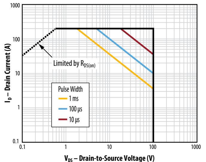
T_J = \text{Max Rated}, T_c = +25^\circ C, \text{Single Pulse}
