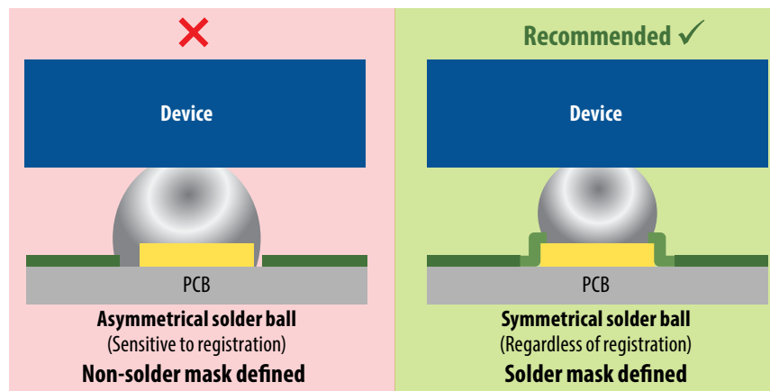
Figure 20: Effect of solder mask design on the solder ball symmetry
