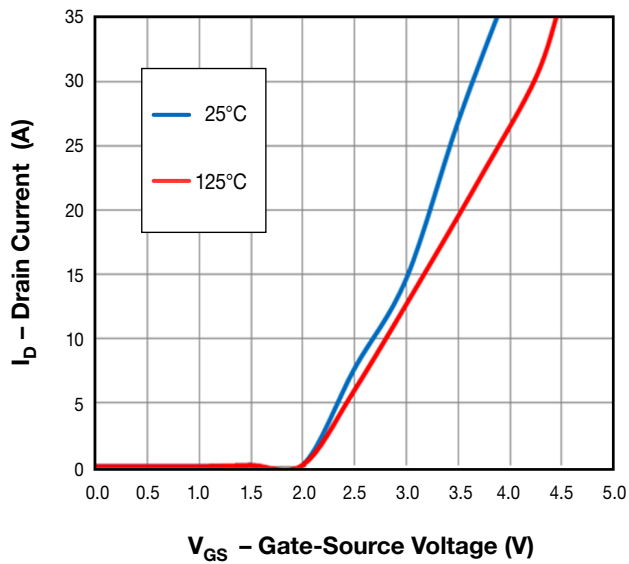
Figure 3. Typical Gate-Drain Transfer Characteristic ( V_{DS} = 3 V)
