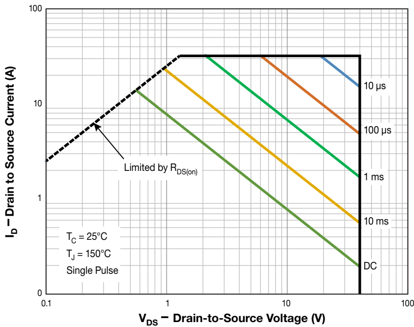
Figure 11. Typical Safe Operating Area
