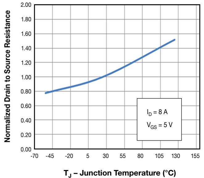
Figure 8. Normalized Drain-Source ON Resistance vs. Ambient Temperature
