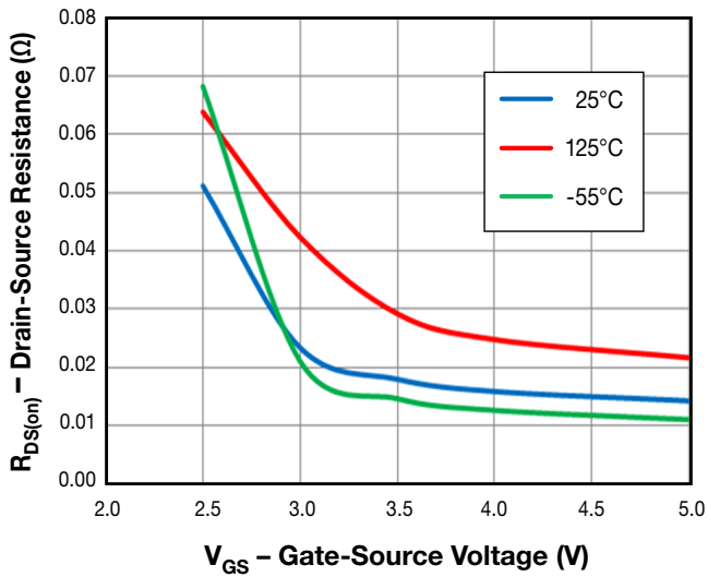
Figure 5. Typical Drain-Source ON Resistance vs. Gate-Source Voltage vs. Temperature
