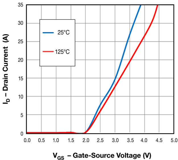
Figure 3. Typical Gate-Drain Transfer Characteristic ( V_{DS} = 3 V)
