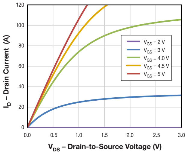
Figure 3. Typical Output Characteristics at 25^\circ\text{C}
