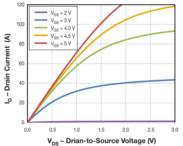
Figure 4. Typical Output Characteristics at 125^\circ\text{C}
