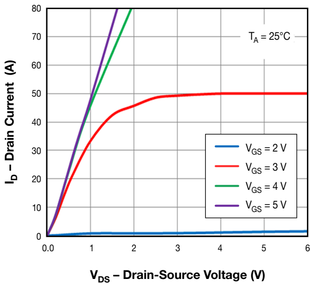
Figure 3. Typical Output Characteristics at 25^\circ\text{C}
