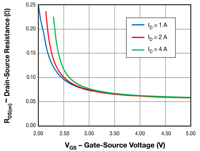
Figure 6. Typical Drain-Source ON Resistance vs. Gate-Source Voltage vs. Drain Current
