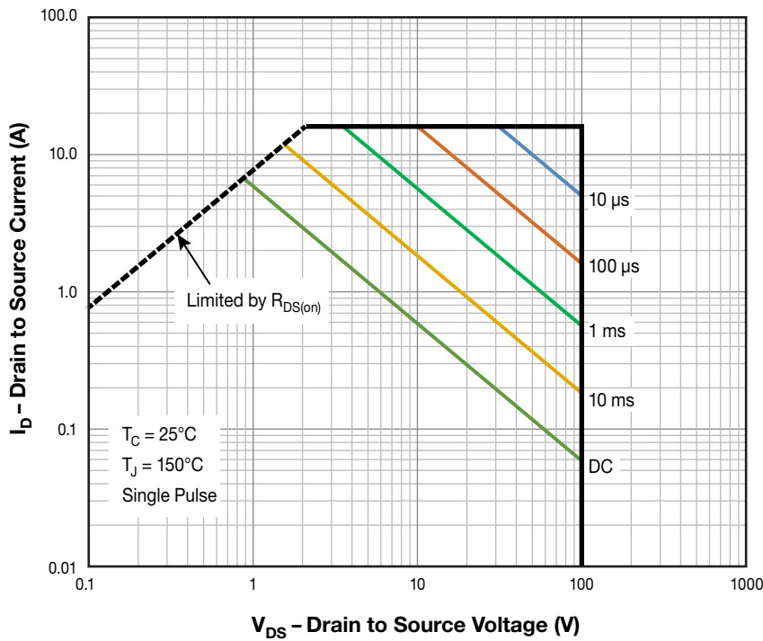
Figure 11. Safe Operating Area
