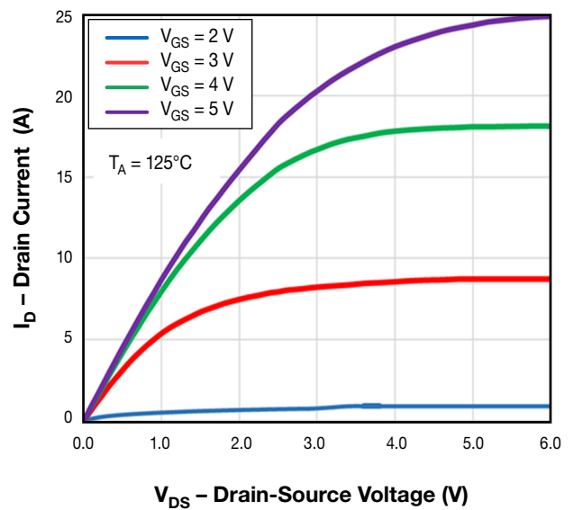
Figure 4. Typical Output Characteristics at 125^\circ\text{C}
