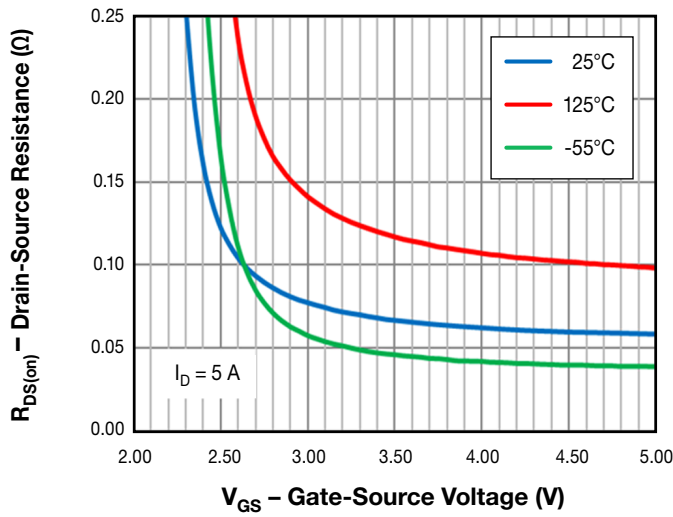
Figure 5. Typical Drain-Source ON Resistance vs. Gate-Source Voltage vs. Ambient Temperature
