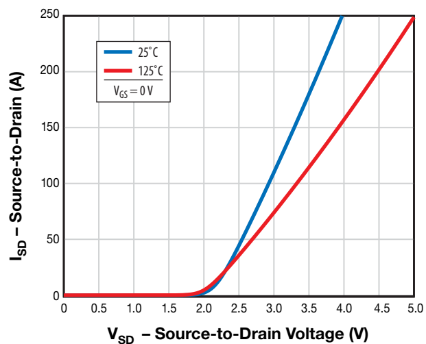
Figure 7. Reverse Drain-Source Characteristics
