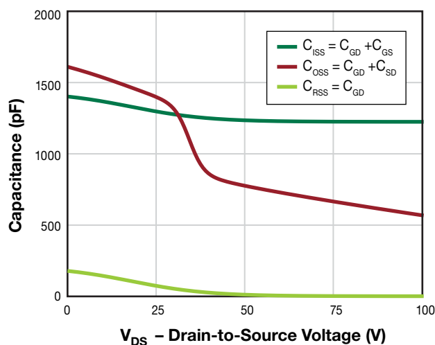
Figure 12. Typical Capacitance
