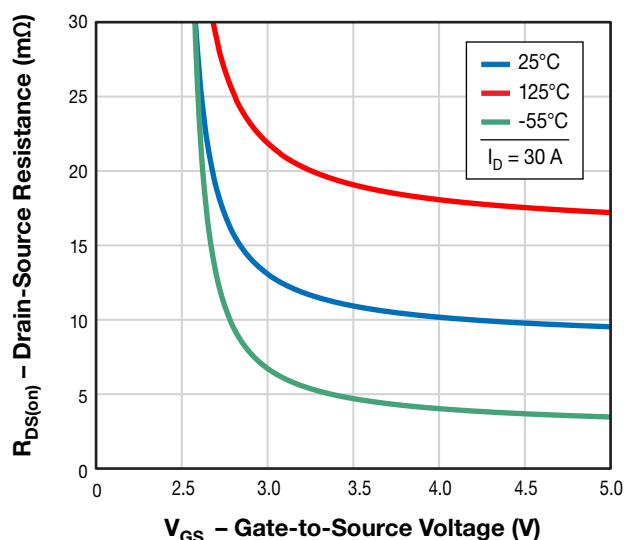
Figure 9. Typical R_{DS(on)} vs. V_{GS} for Various Temperatures
