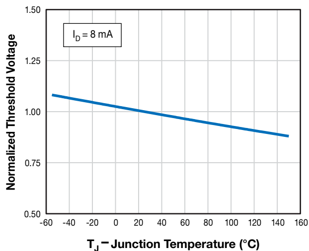
Figure 11. Normalized Threshold Voltage vs. Temperature
