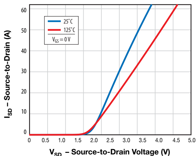
Figure 7. Reverse Drain-Source Characteristics
