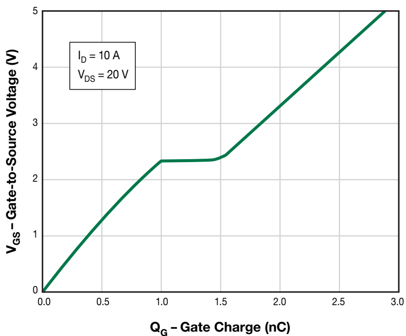
Figure 14. Typical Gate Charge
