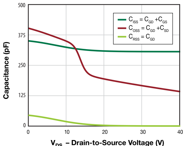
Figure 12. Typical Capacitance
