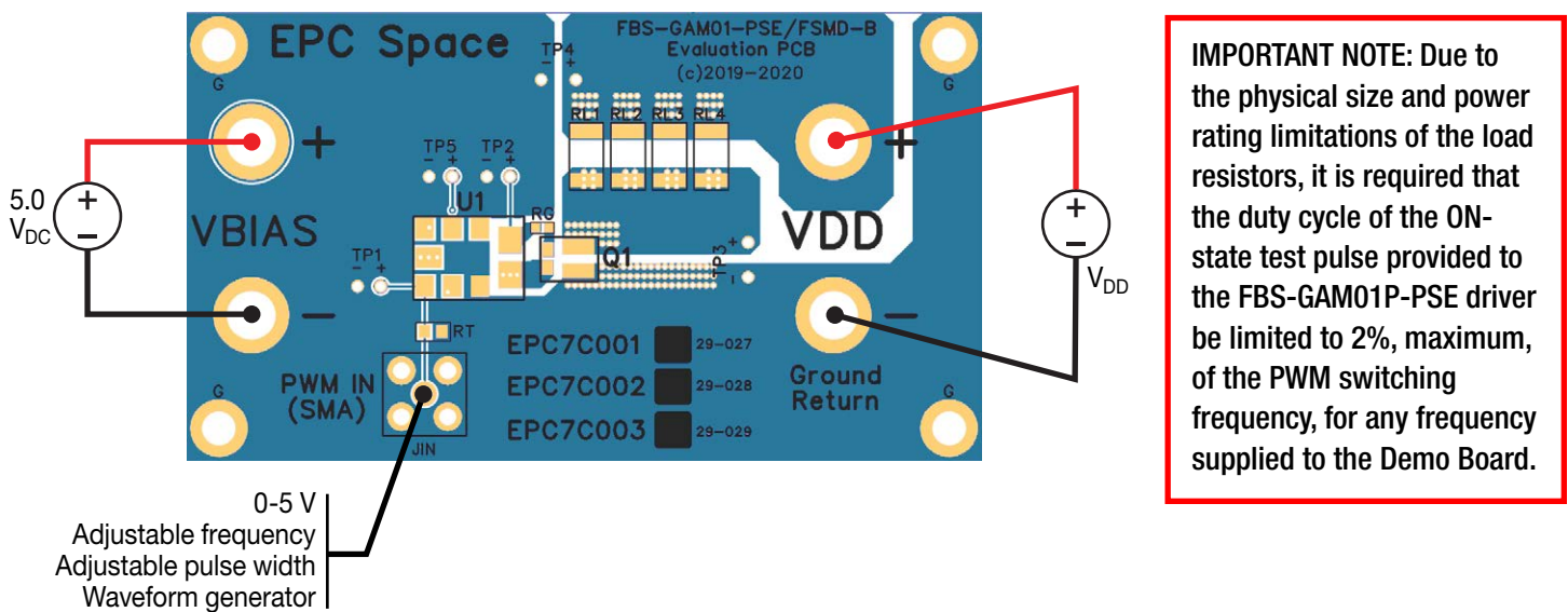
Figure 2. EPC7C003 Demo Board Test Equipment Connections
