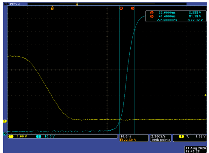
Figure 6. FBG20N18 t_f
