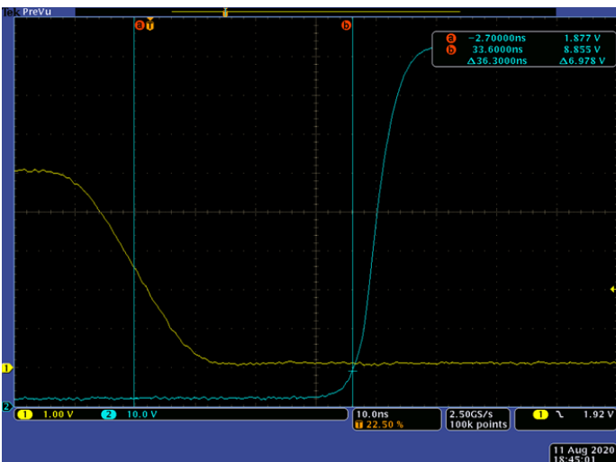
Figure 5. FBG20N18 t_{d(OFF)}
