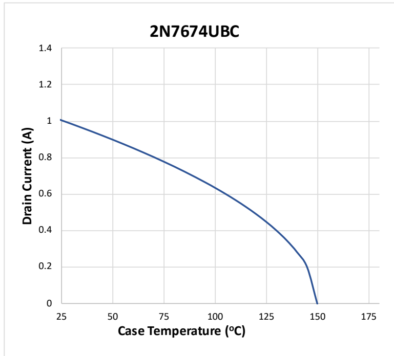
FIGURE 5. Drain Current vs Temperature graph.
