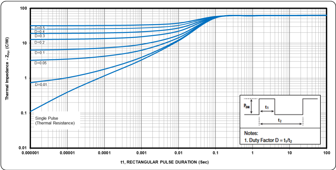
FIGURE 3. Thermal impedance graph.
